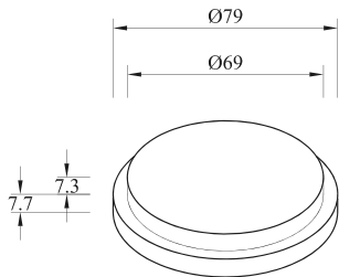
2RH.36 Blanking Cap Teak
