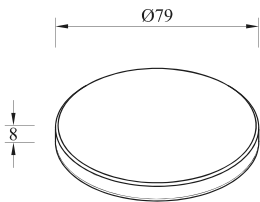
4PR.00 / 4PRSS.00 Blanking Cap Brass and Stainless Steel
