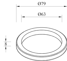
4PR.61 / 4PRSS.61 Reducer Ring Brass and Stainless Steel
