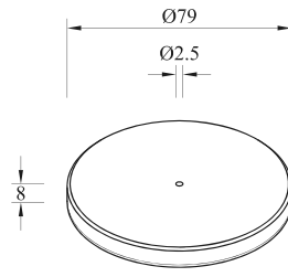
F-APC-/.01/.02/.04 Blanking Cap for Cayman Tables
